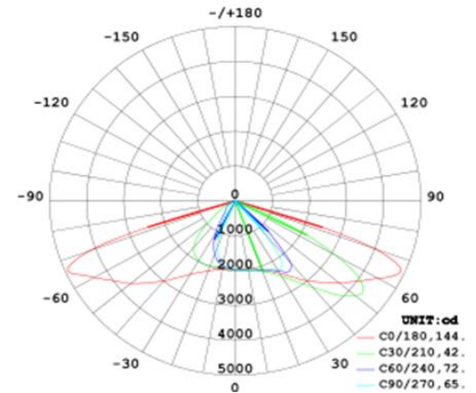
Light Distribution Curve
