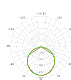
Housing 4inch
