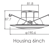
Housing 6inch
